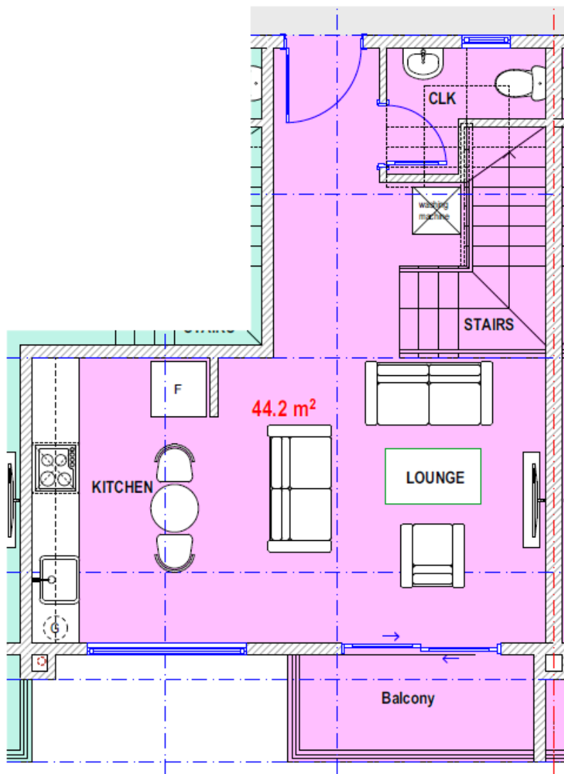
1 BED DUPLEX TYPE 2B - LOWER FLOOR
