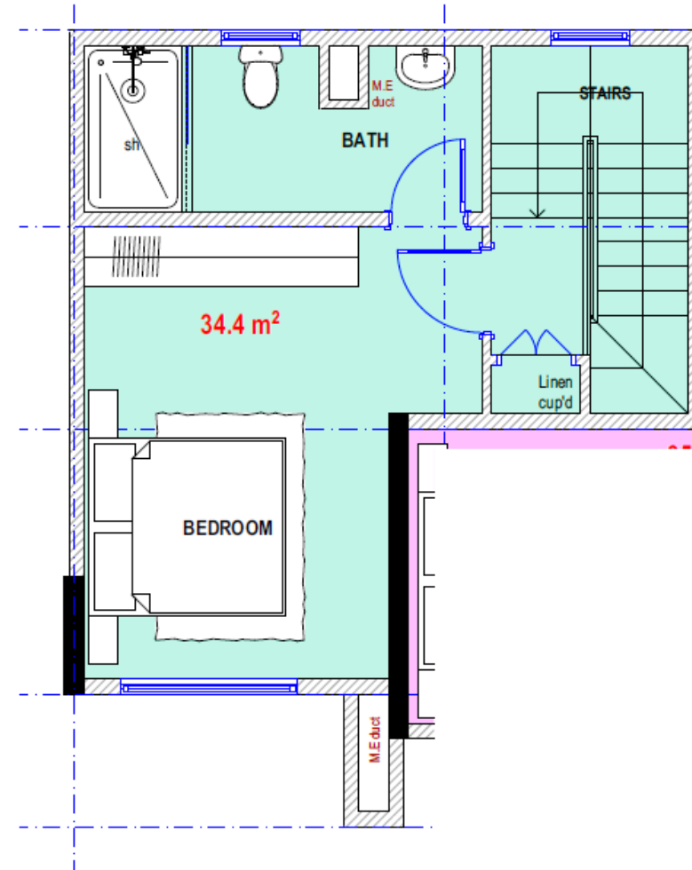
1 BED DUPLEX - TYPE 1 UPPER LAYOUT
