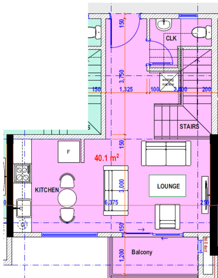
1 BED DUPLEX - TYPE 2 LOWER LAYOUT
