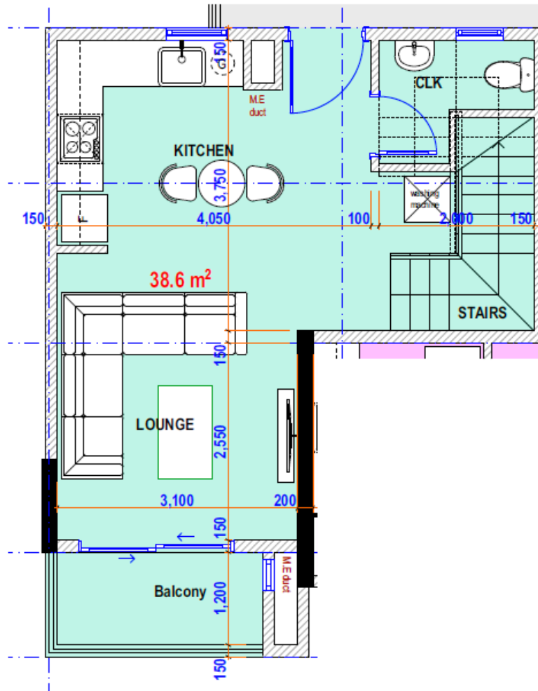
1 BED DUPLEX - TYPE 1 LOWER LAYOUT
