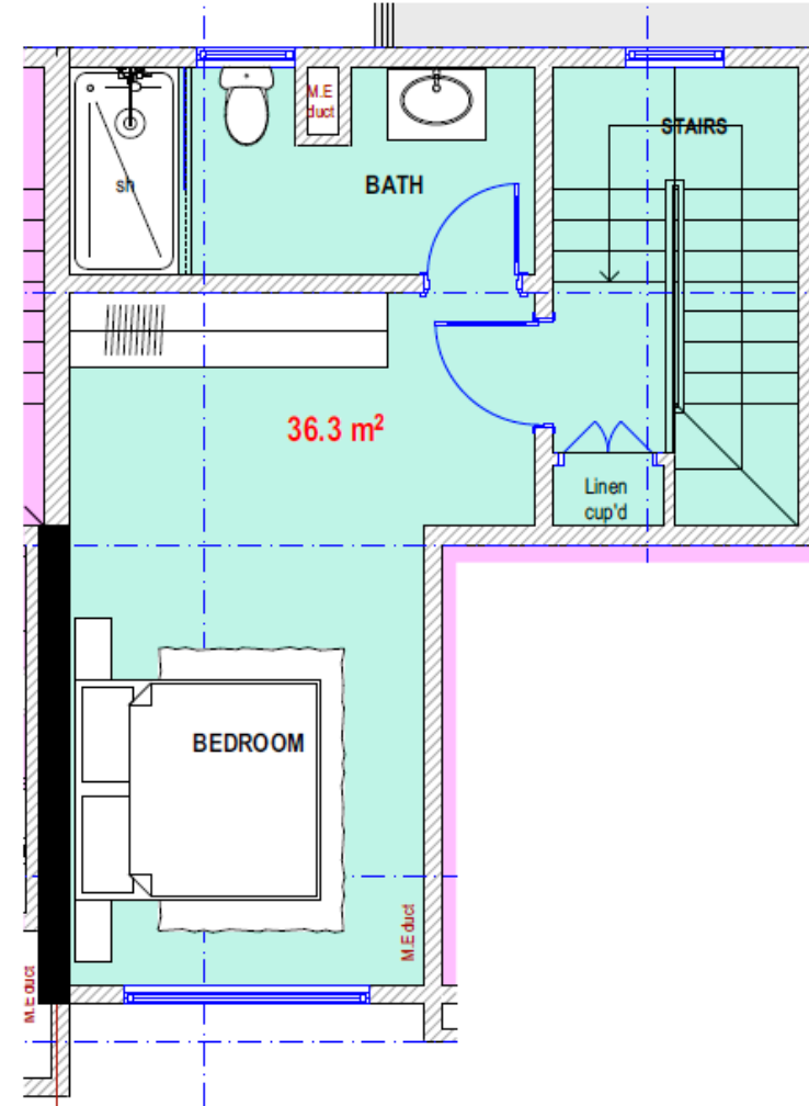
1 BED DUPLEX TYPE 1B - UPPER FLOOR
