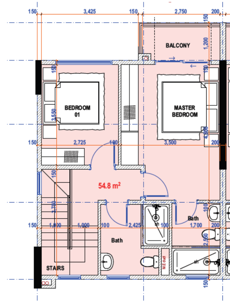
2 BED DUPLEX UPPER FLOOR
