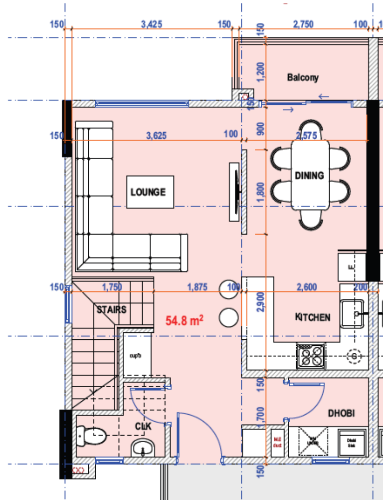
2 BED DUPLEX LOWER FLOOR
